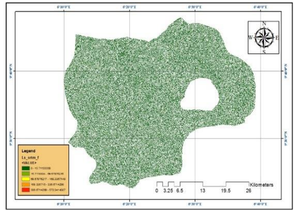
Figure 3. Slope length and steepness factor map of the study area
