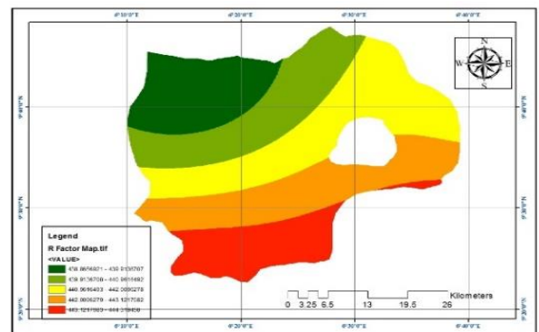
Figure 1. Rainfall erosivity factor map
