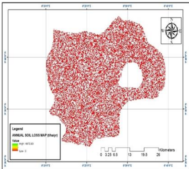
Figure 5. Mean annual soil loss map
