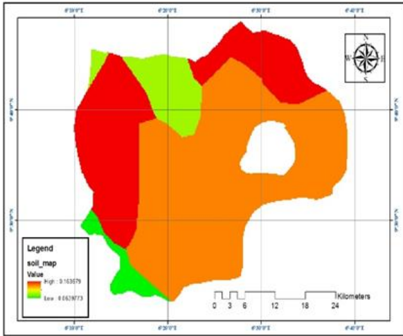
Figure 2. Soil erodibility factor map of Bosso local government Area
