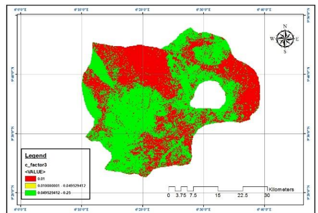
Figure 4. Conservation factor map
